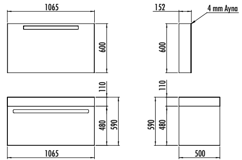
RE0105.42 Recta Lavabo Dolabı 105 cm (1065x590x500 mm) (GxYxD) RE1105.42 Recta LED'li Aynalı Dolap 105 cm (1065x600x150 mm) (GxYxD)
