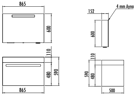
RE0085.42 Recta Lavabo Dolabı 85 cm (865x590x500 mm) (GxYxD) RE1085.42 Recta LED'li Aynalı Dolap 85 cm (865x600x150 mm) (GxYxD)
